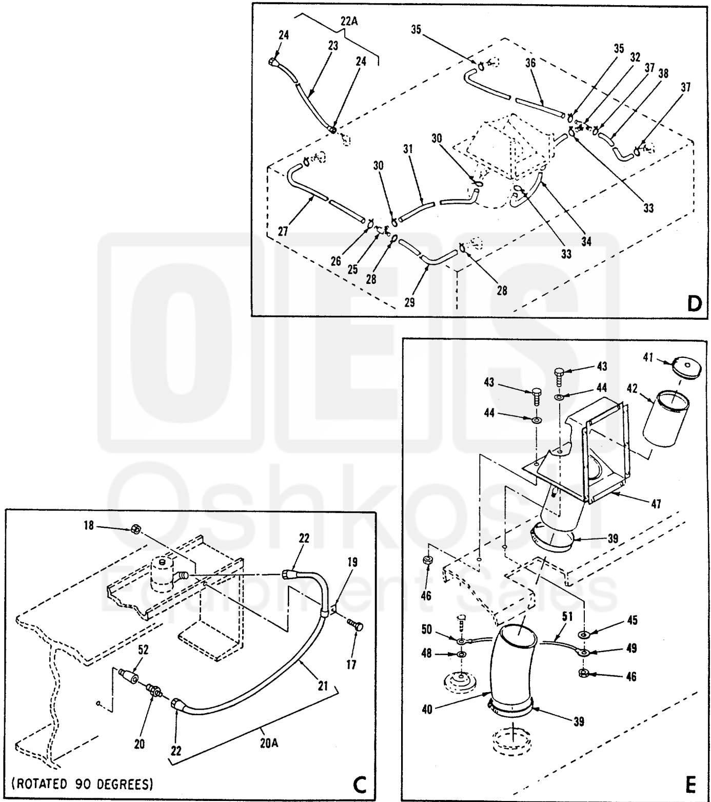
Figure 41. Fuel Line Assembly (Sheet 2 of 2)
